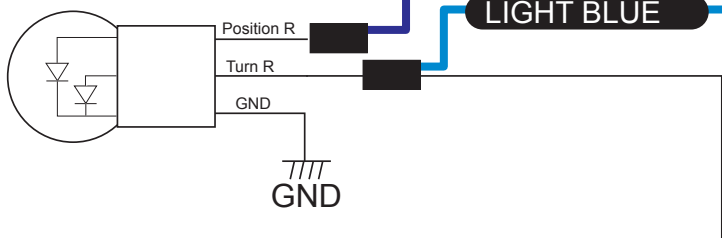
Front LED 2function winker R
