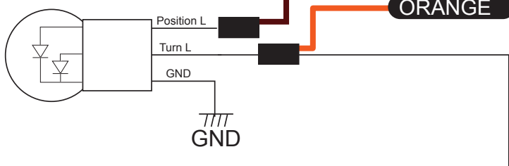
Front LED 2function winker L
